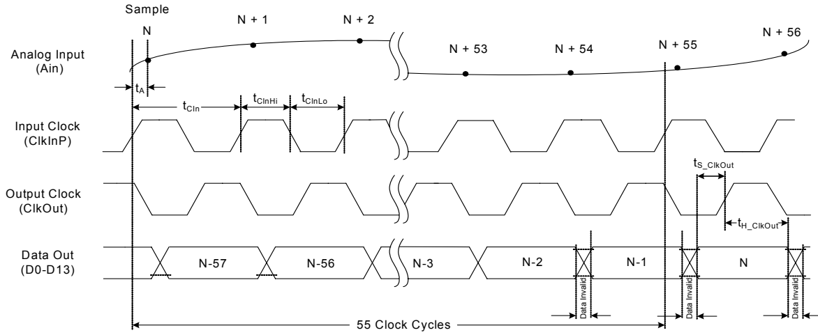
Figure 1. Timing Diagram
