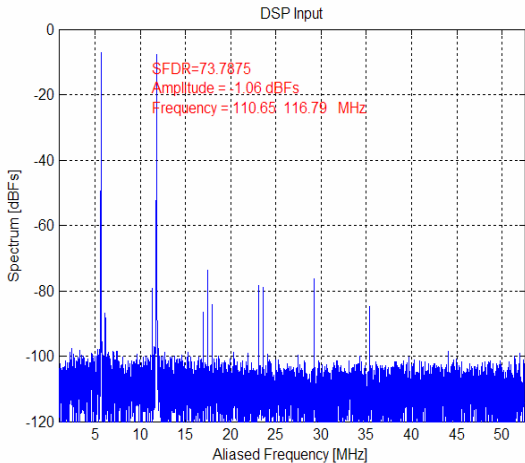
Figure 4. Two Tone (110.7, 116.8MHz) Before Linearization SFDR 73.8dB (typ)
